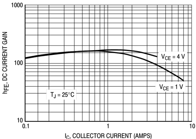
Figure 4. MJF44H11 DC Current Gain
