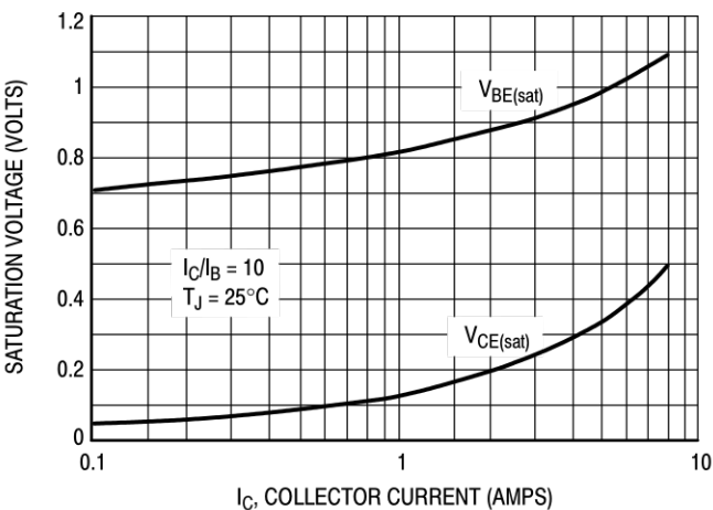
Figure 9. MJF45H11 On-Voltages
