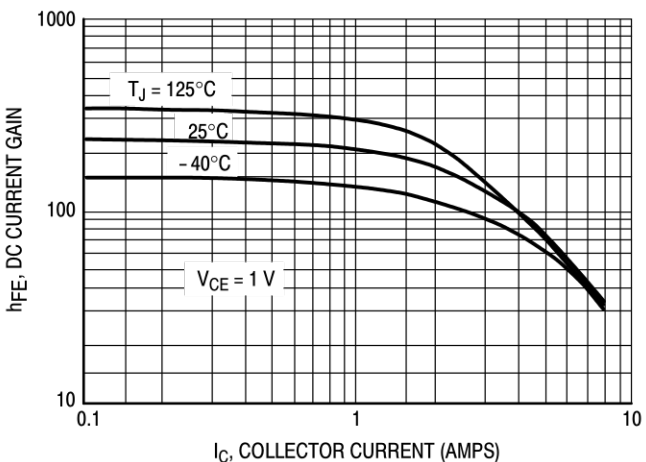
Figure 7. MJF45H11 Current Gain versus Temperature
