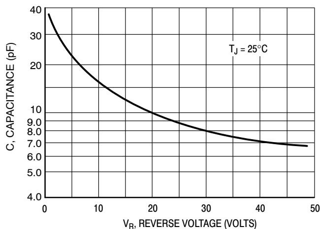
Figure 10. Typical Capacitance
