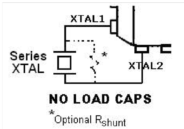
Figure 8. Crystal Application
