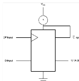
FIGURE 2. I_{CCD} Test Circuit
