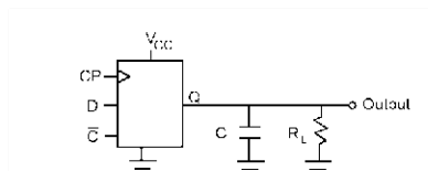
FIGURE 1. AC Test Circuit
