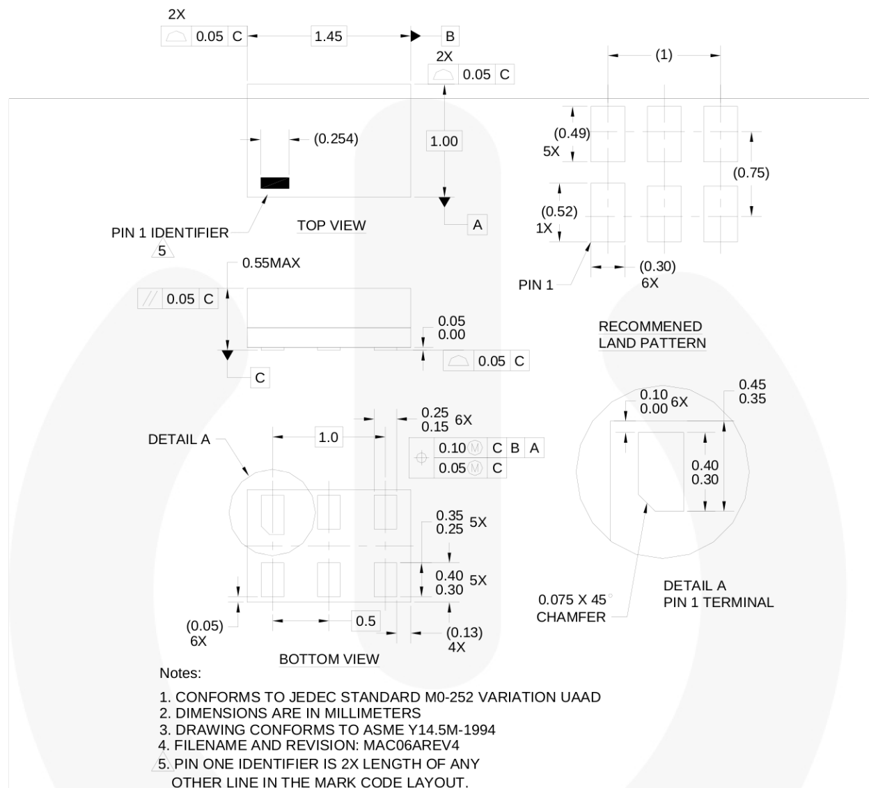
Figure 18. 6-Lead, MicroPak™, 1.0mm Wide
