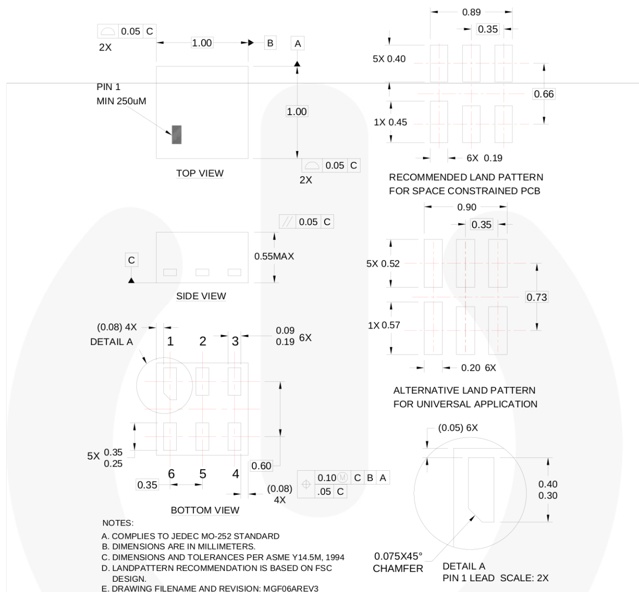
Figure 19. 6-Lead, MicroPak2™, 1x1mm Body, .35mm Pitch
