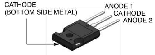
TO-247-3LD CASE 340CK
