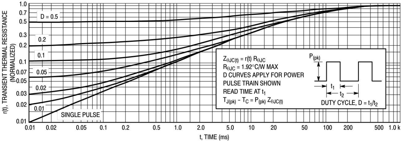
Figure 5. Thermal Response
