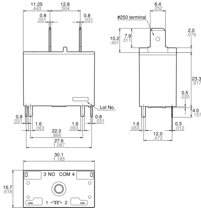
External dimensions
