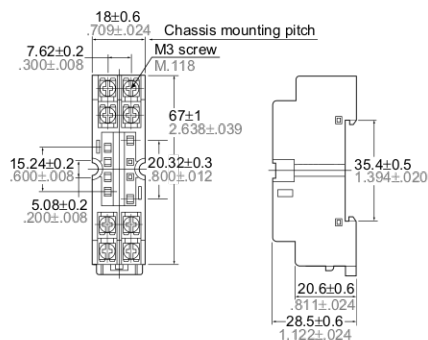
External dimensions
