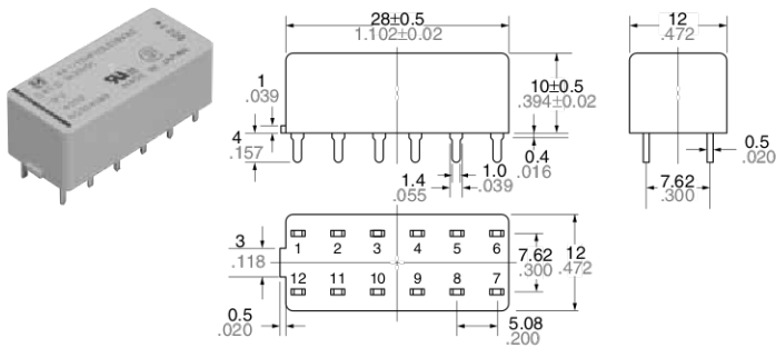
External dimensions
