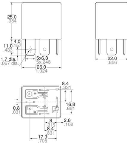
External dimensions
