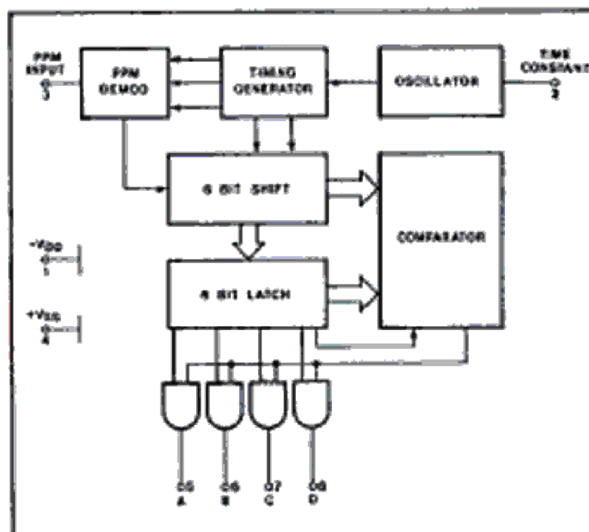
Fig. 2 Block diagram
