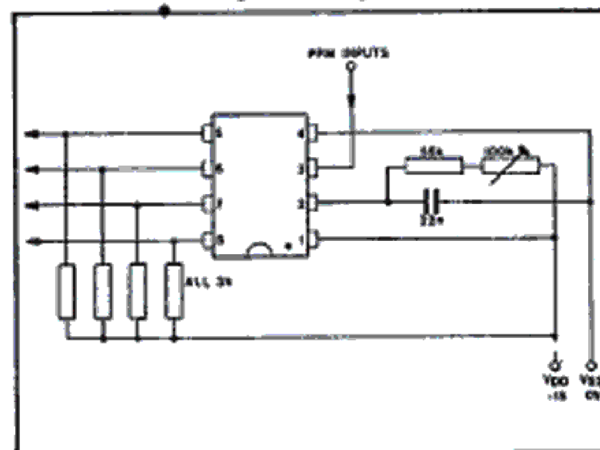
Fig. 3 Test circuit
