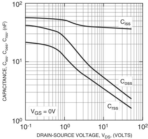
CAPACITANCE VS. DRAIN-SOURCE VOLTAGE (TYPICAL)
