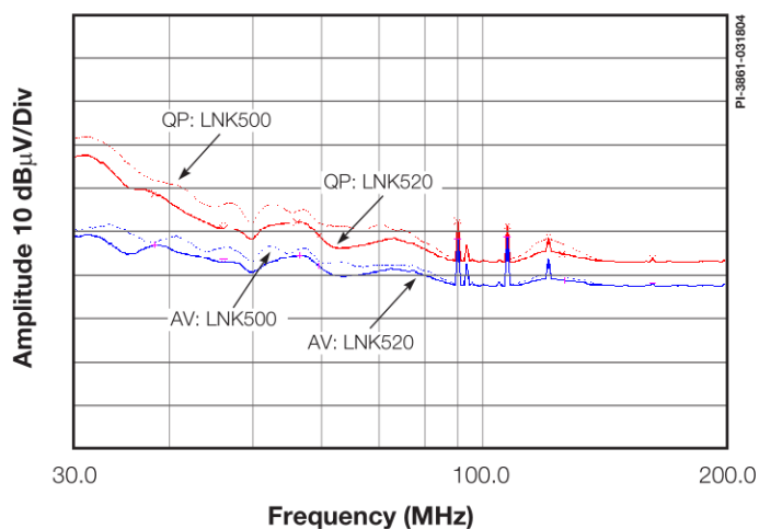
Figure 13. Comparison of LNK520 and LNK500 Showing an Approximate 5 dB \mu V Reduction in Radiated EMI.
