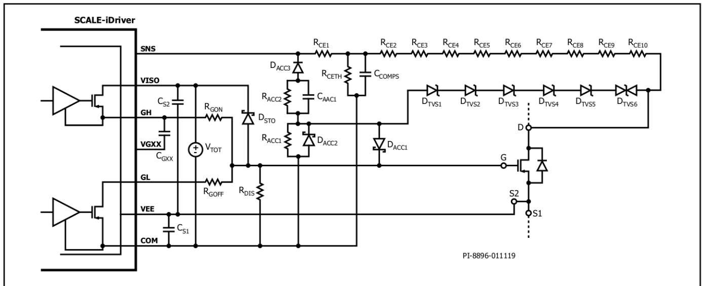
Figure 8. Secondary-Side of Example Circuitry.
