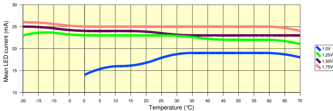
Mean LED Current vs. Temp. @ L1=10 \mu H
