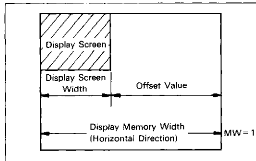
Figure 11 Memory Width
