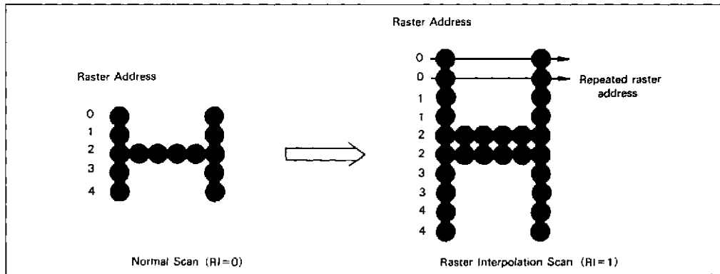
Figure 14 Raster Interpolation
