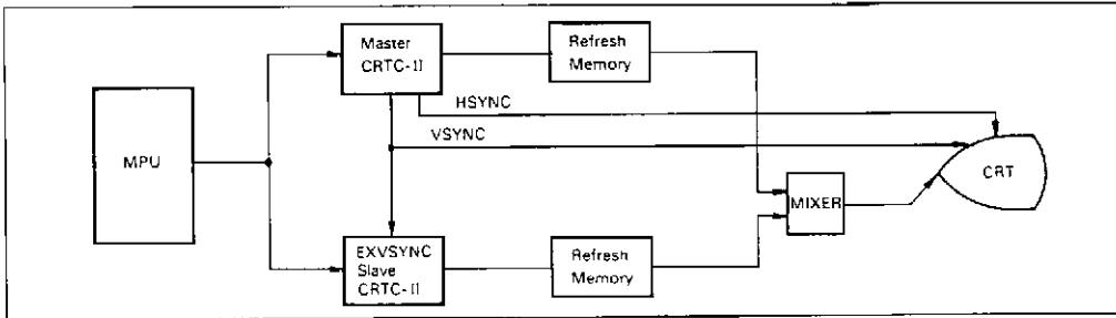
Figure 16 Master-Slave Mode
