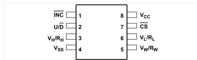
X9C102, X9C103, X9C104, X9C503 (8 LD SOIC, 8 LD PDIP) TOP VIEW
