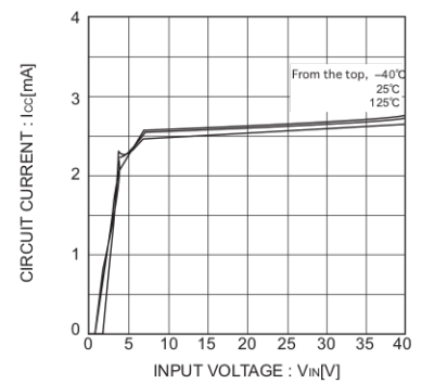
Fig.6 Circuit current(BD9781HFP)
