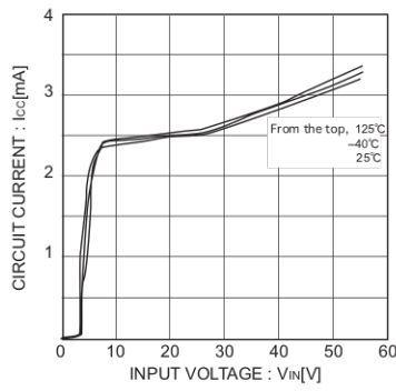
Fig.8 Circuit current(BD9001F)
