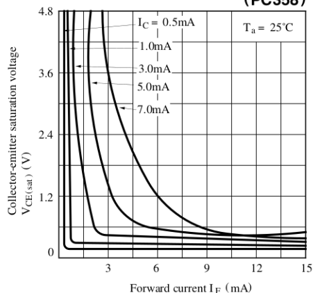
Fig.13-b Collector-emitter Saturation Voltage vs. Forward Current (PC358)
