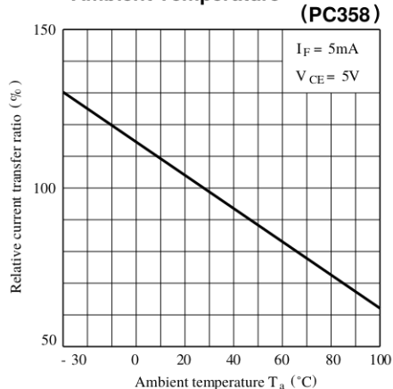
Fig. 9-b Relative Current Transfer Ratio vs. Ambient Temperature (PC358)
