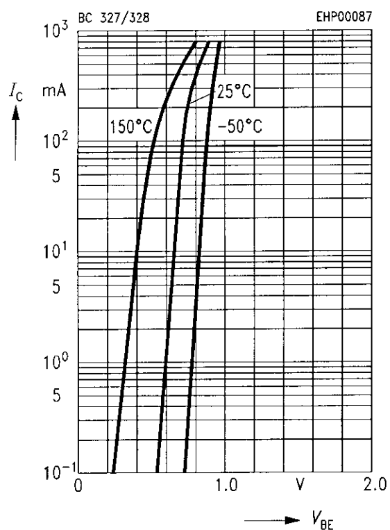
Collector current I_C = f(V_{\text{BE}})
