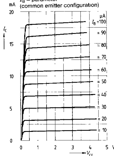
Output characteristics Collector current versus collector-emitter voltage I_B = parameter (common emitter configuration)
