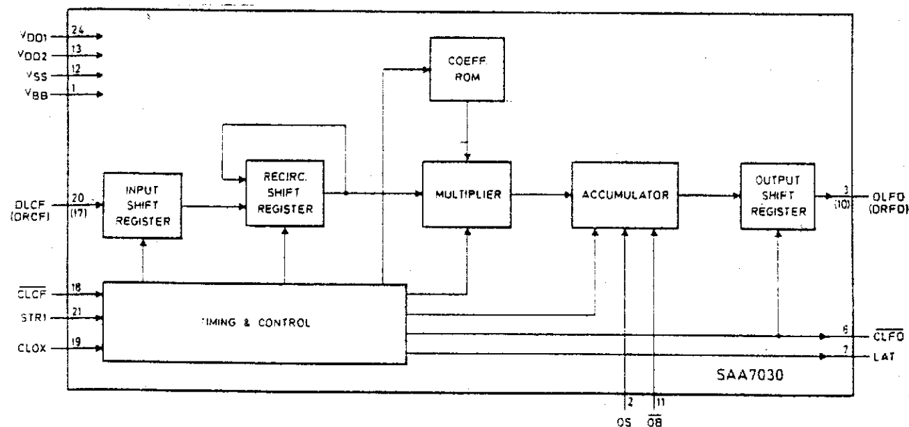
Fig. 1 Block diagram.
