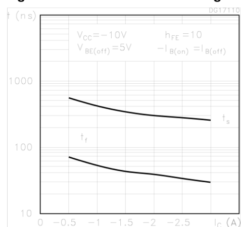
Figure 7. Resistive load switching off
