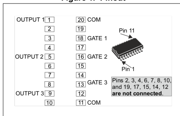
Figure 1. Pinout
