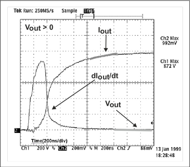
Figure 20. Current and voltage of the ACS during IEC 61000-4-5 standard test with R = 150\ \Omega , L = 5\ \mu\text{H} , V_{PP} = 2\ \text{kV}
