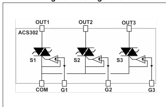
Figure 2. Configuration
