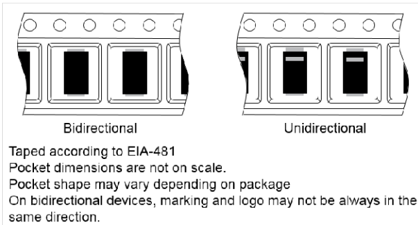
Figure 16. Package orientation in reel
