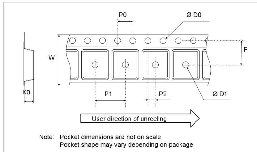
Figure 20. Tape outline
