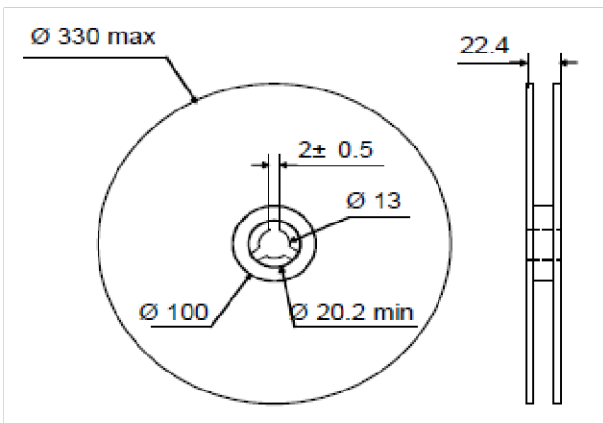
Figure 18. 13" reel dimension values (mm)
