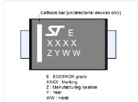
Figure 15. Marking layout
