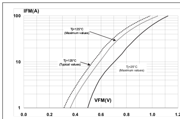
Figure 5. Forward voltage drop vs. forward current (per diode)
