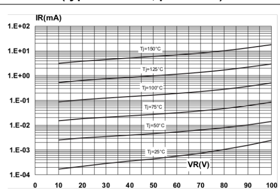
Figure 6. Reverse leakage current versus reverse voltage applied (typical values, per diode)
