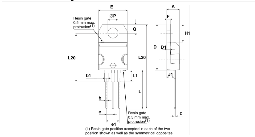
Figure 11. TO-220AB dimension definitions
