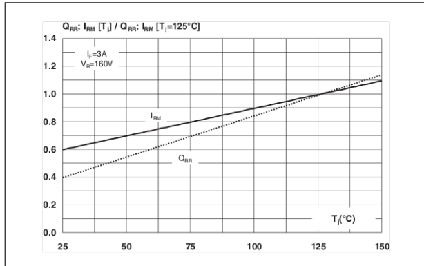
Figure 11. Dynamic parameters versus junction temperature
