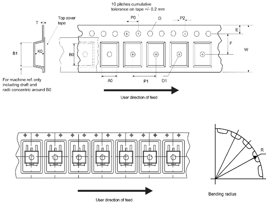
Figure 36. DPAK tape
