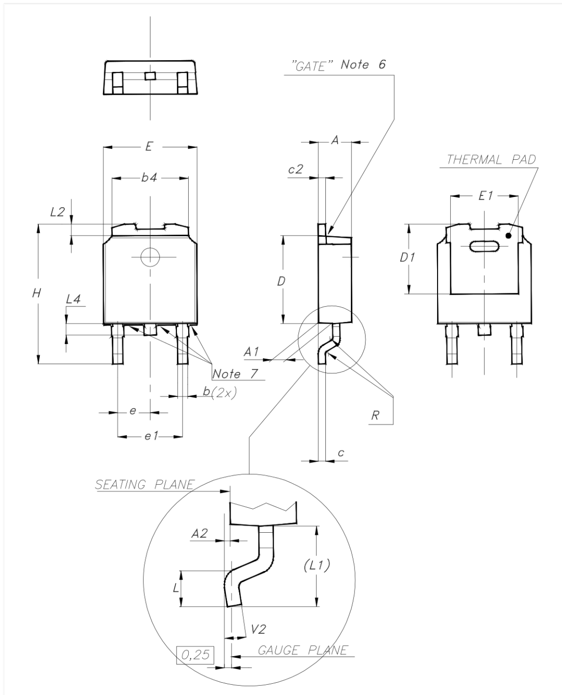
Figure 32. DPAK (TO-252) package outline A
