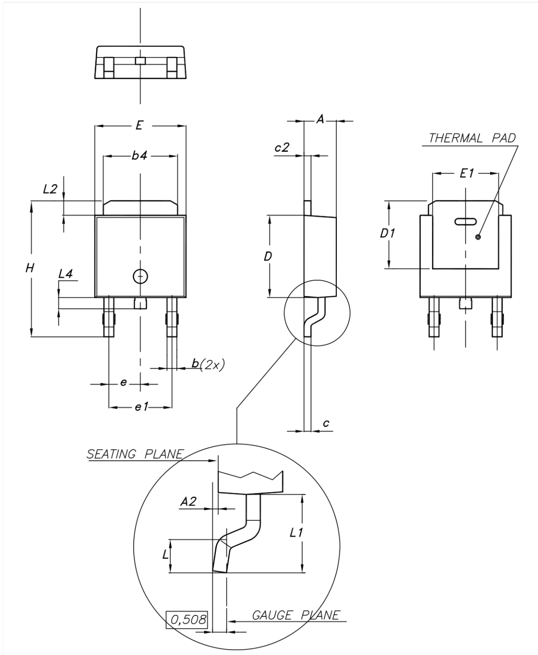
Figure 33. DPAK (TO-252) package outline E
