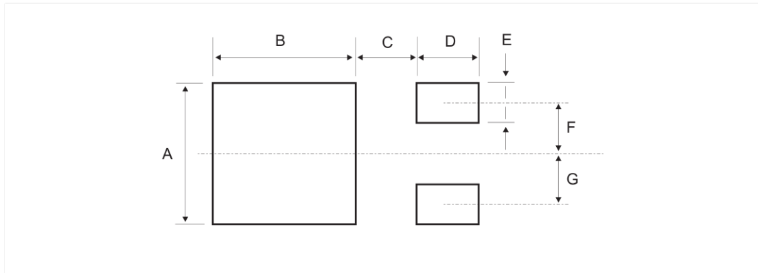
Figure 35. DPAK footprint recommended data
