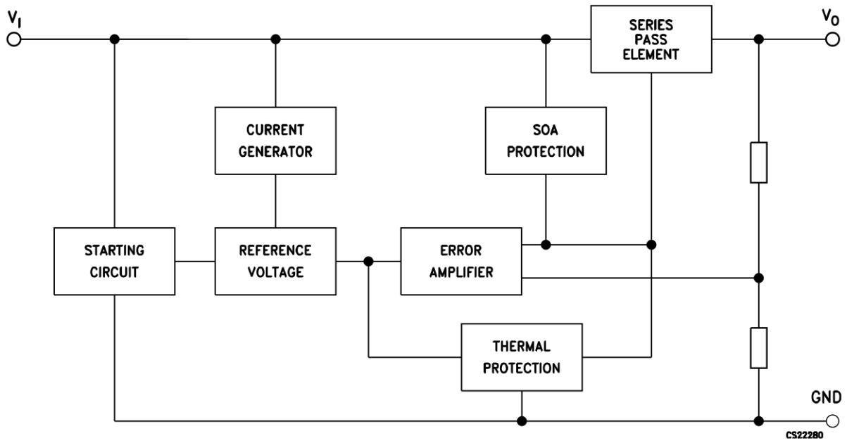
Figure 1. Block diagram
