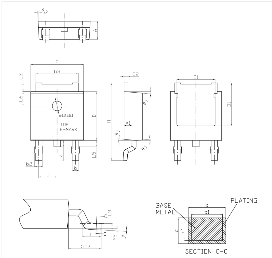
Figure 34. DPAK (TO-252) package outline I
