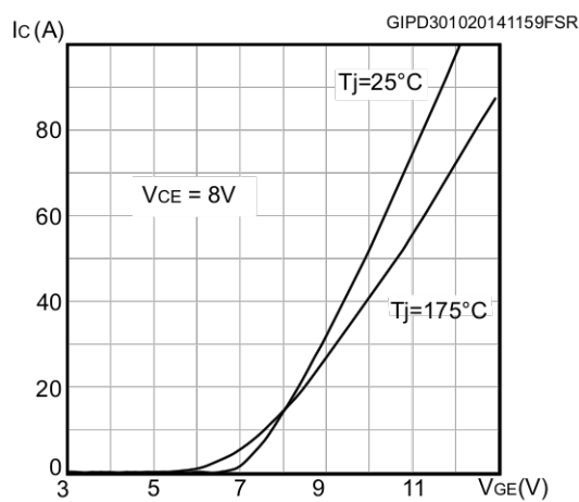
Figure 9. Transfer characteristics
