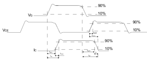
Figure 30. Switching waveform
