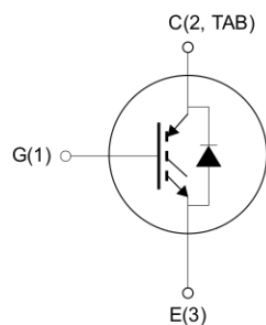
TO-247
