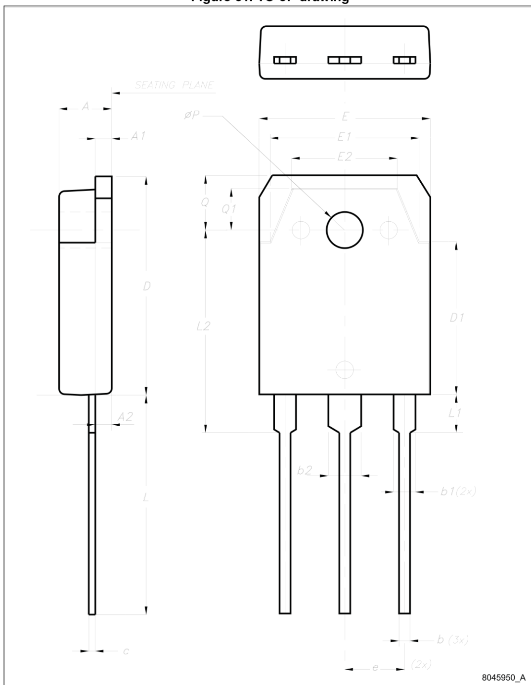
Figure 31. TO-3P drawing
