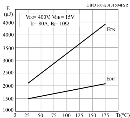
Figure 17. Switching energy vs temperature
