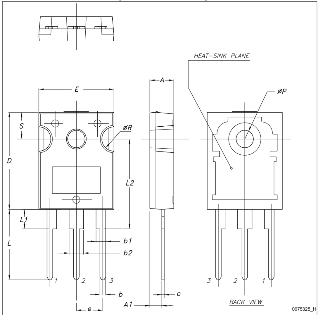
Figure 29. TO-247 drawing
