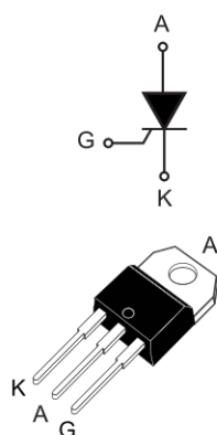
TO-220AB
