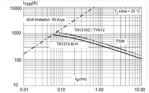
Figure 8. Non repetitive surge peak on-state current for a sinusoidal pulse with width t_p < 10\text{ ms}
