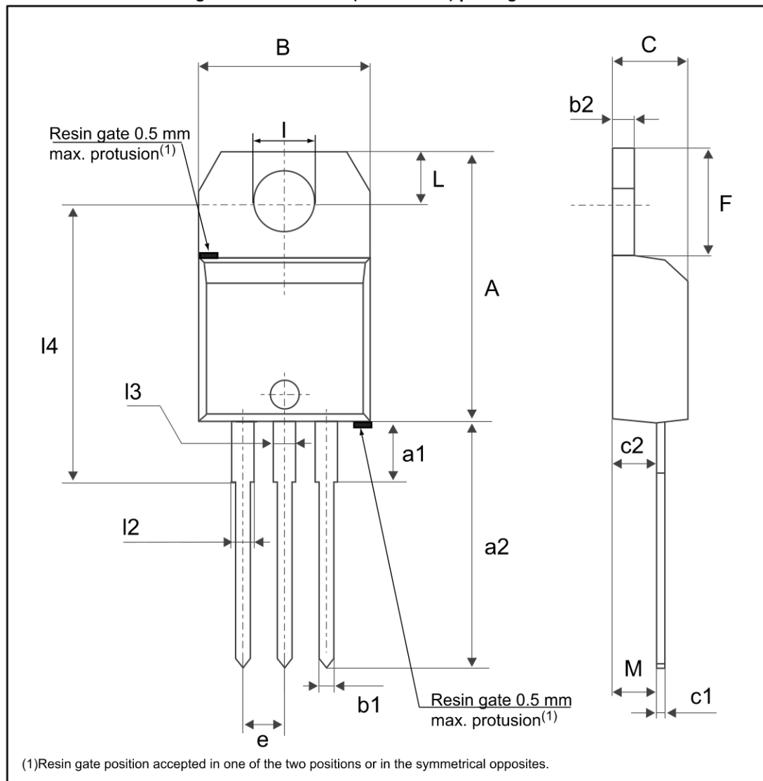
Figure 12: TO-220AB (Nlms. & Ins.) package outline
