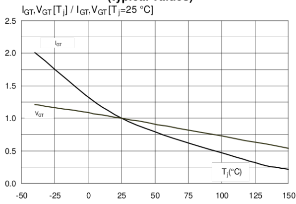
Figure 5: Relative variation of gate trigger current and gate voltage versus junction temperature (typical values)
