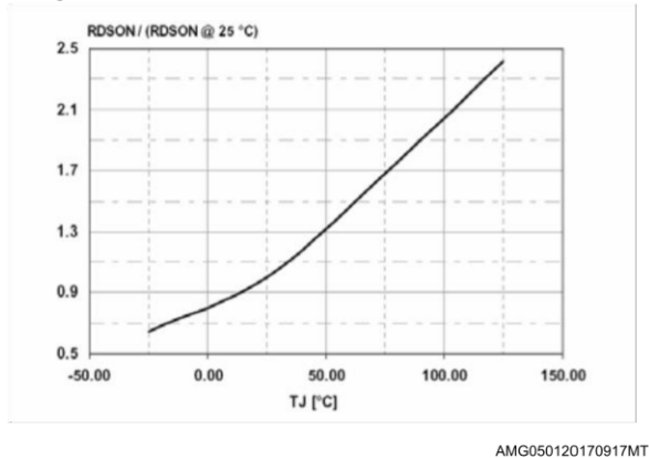
Figure 17: Power MOSFET on-resistance vs T_J
