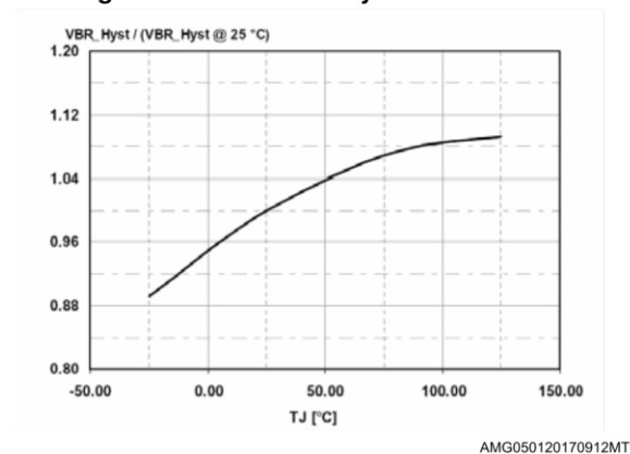
Figure 12: Brown out hysteresis vs T_J
