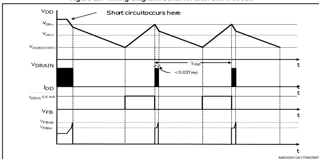
Figure 25: Timing diagram: behavior after short circuit
