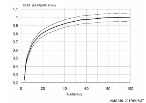
Figure 16: Current limit vs R_{LM}
