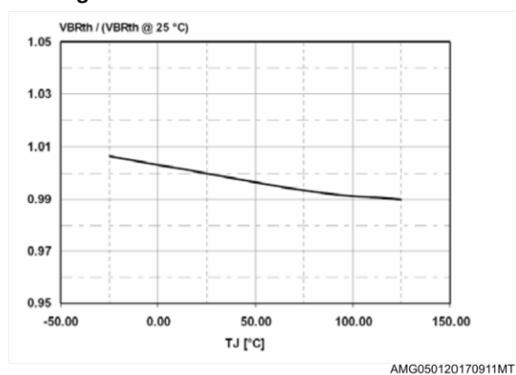
Figure 11: Brown out threshold vs T_J
