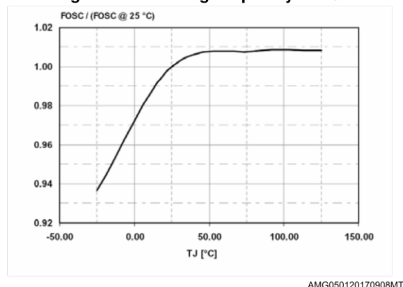
Figure 8: Switching frequency vs T_J
