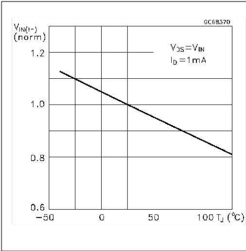
Figure 28. Normalized Input threshold voltage Vs. temperature
