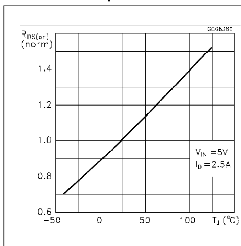
Figure 14. Normalized on resistance Vs temperature
