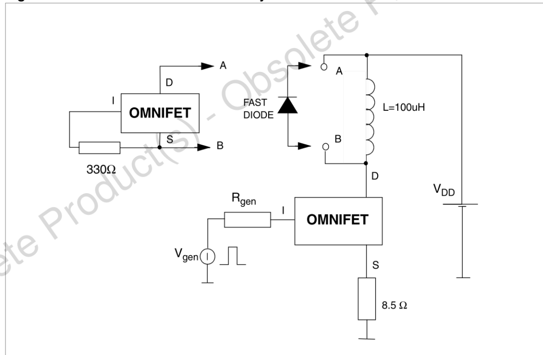
Figure 3. Test circuit for diode recovery times
