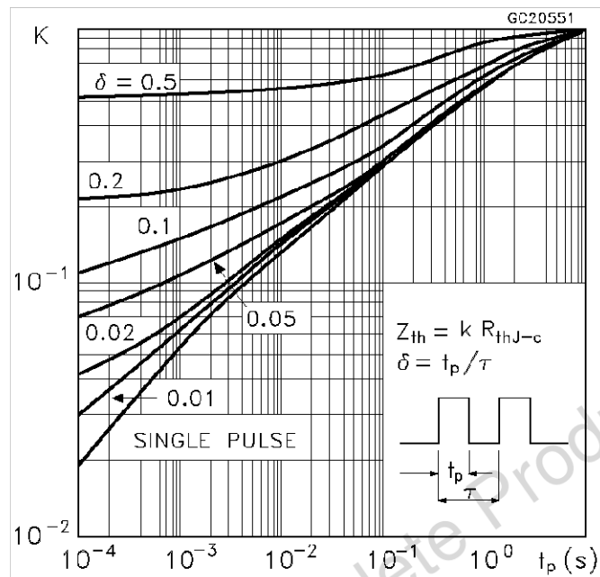
Figure 8. Thermal impedance for ISOWATT220
