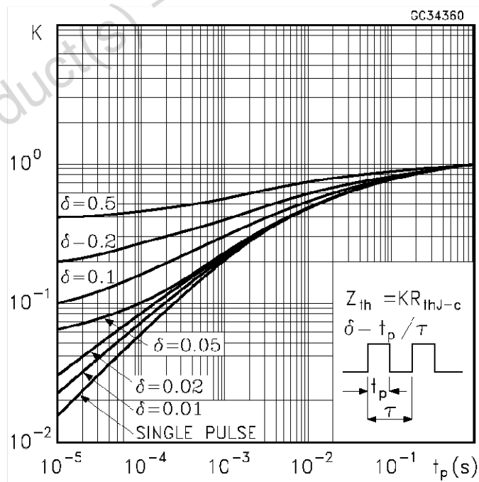
Figure 9. Thermal impedance for DPAK / IPAK
