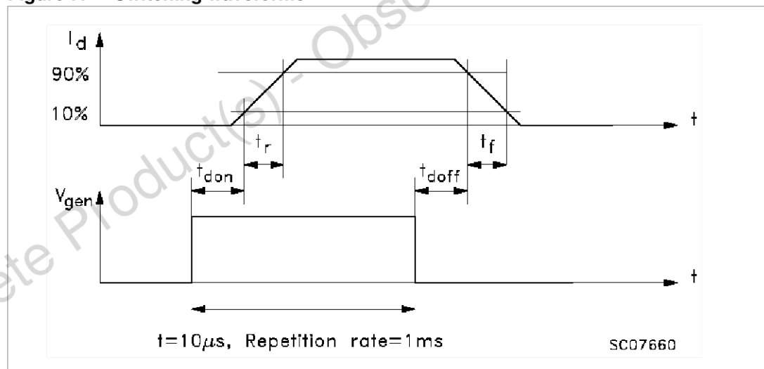
Figure 7. Switching waveforms
