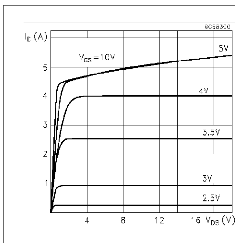
Figure 26. Output characteristics
