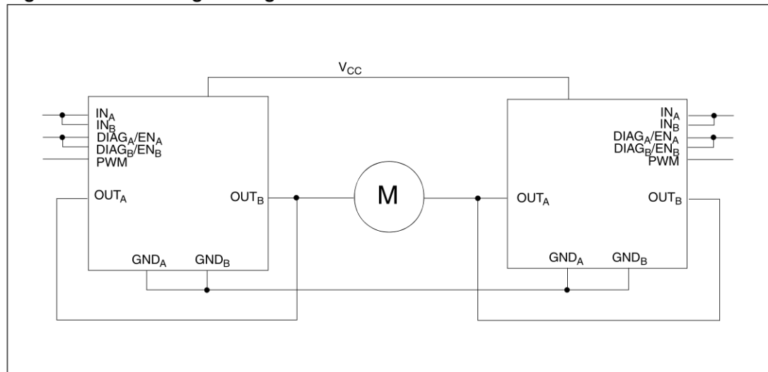
Figure 34. Half-bridge configuration
