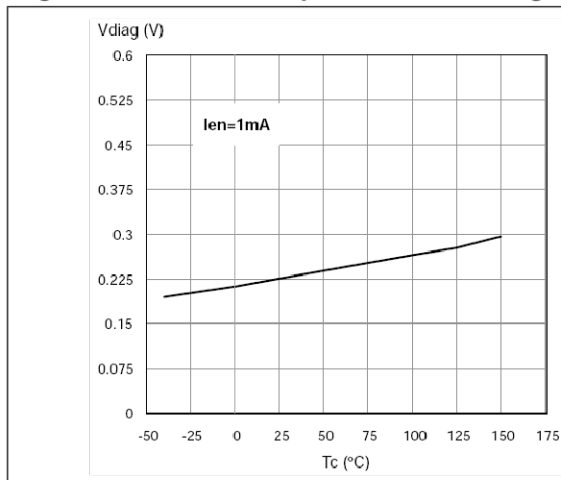
Figure 31. Enable output low level voltage
