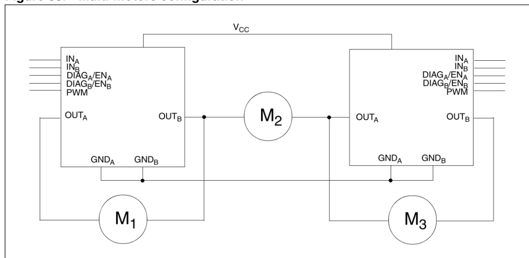
Figure 35. Multi-motors configuration
