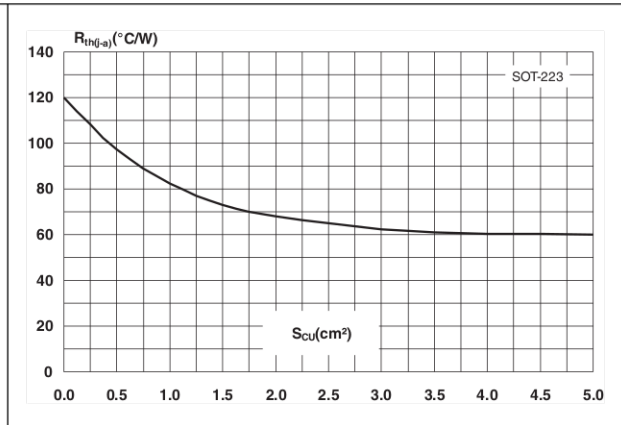
Figure 8. SOT-223 junction to ambient thermal resistance versus copper surface under tab (PCB FR4, copper thickness 35 \mu\text{m} )
