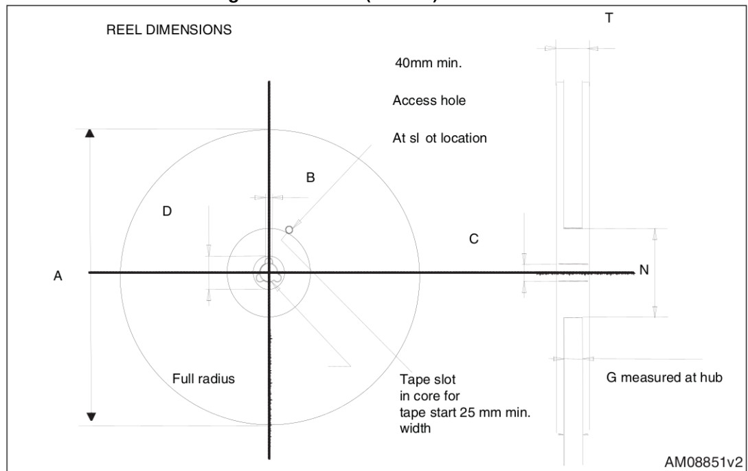
Figure 29. D 2 PAK (TO-263) reel outline
