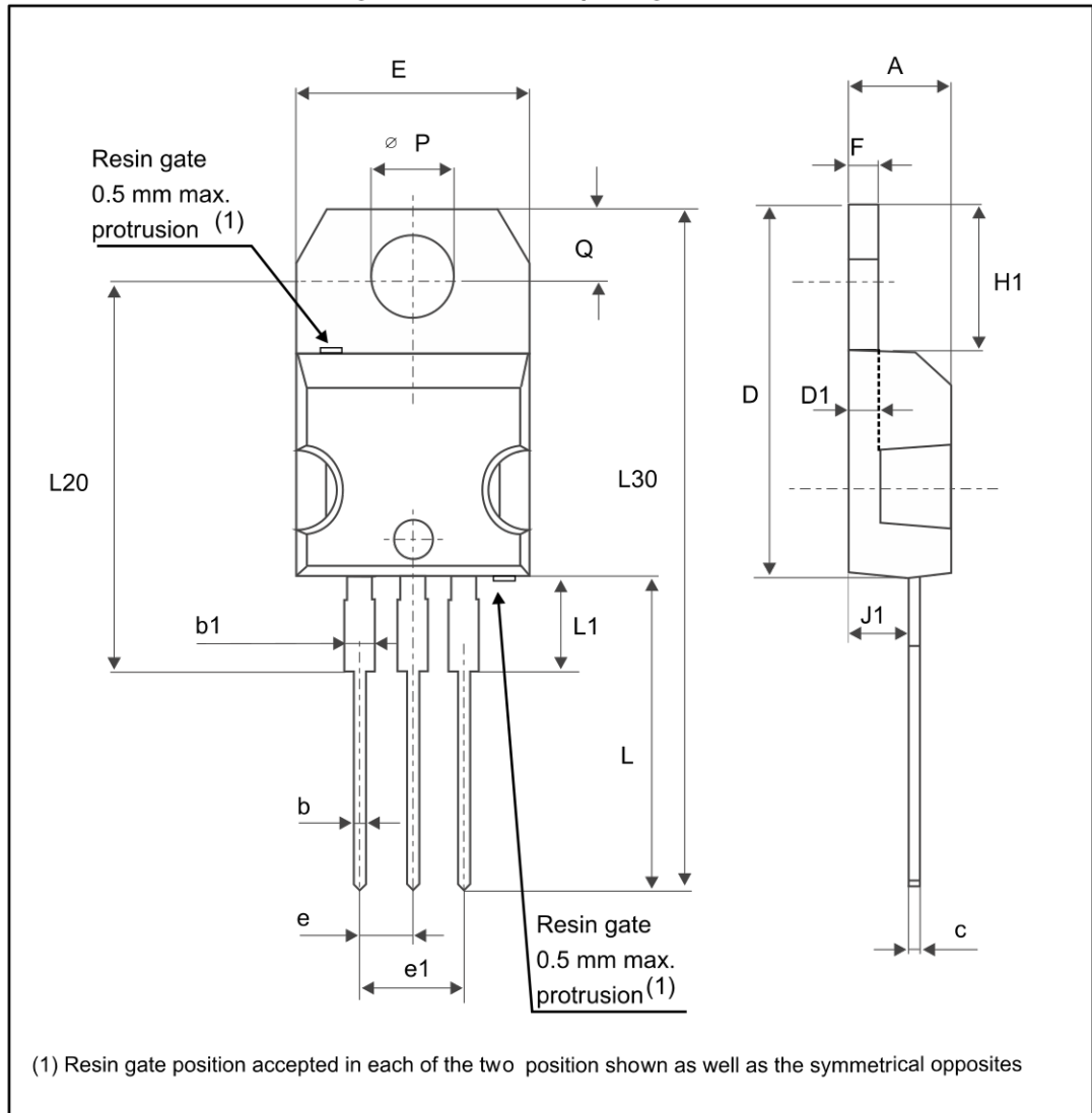
Figure 16: TO-220AB package outline
