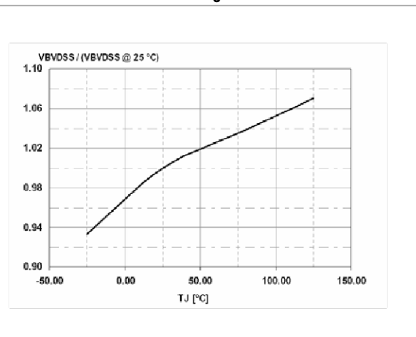
Figure 15. Power MOSFET break down voltage vs T_J
