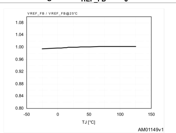
Figure 9. V_{REF\_FB} vs T_J
