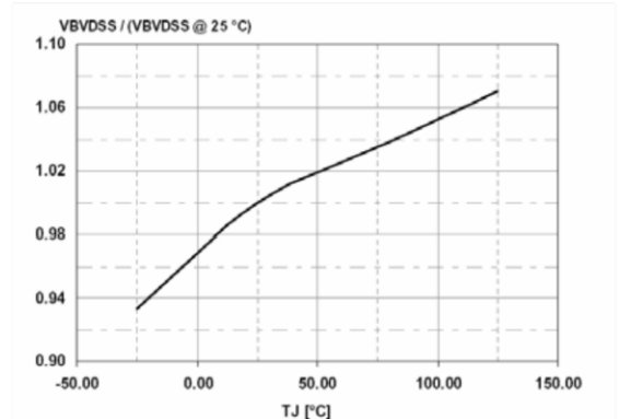
Figure 18: Power MOSFET break down voltage vs T_J
