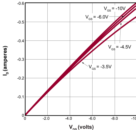
Saturation Characteristics
