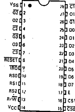
FIGURE 1 - PIN ASSIGNMENT
