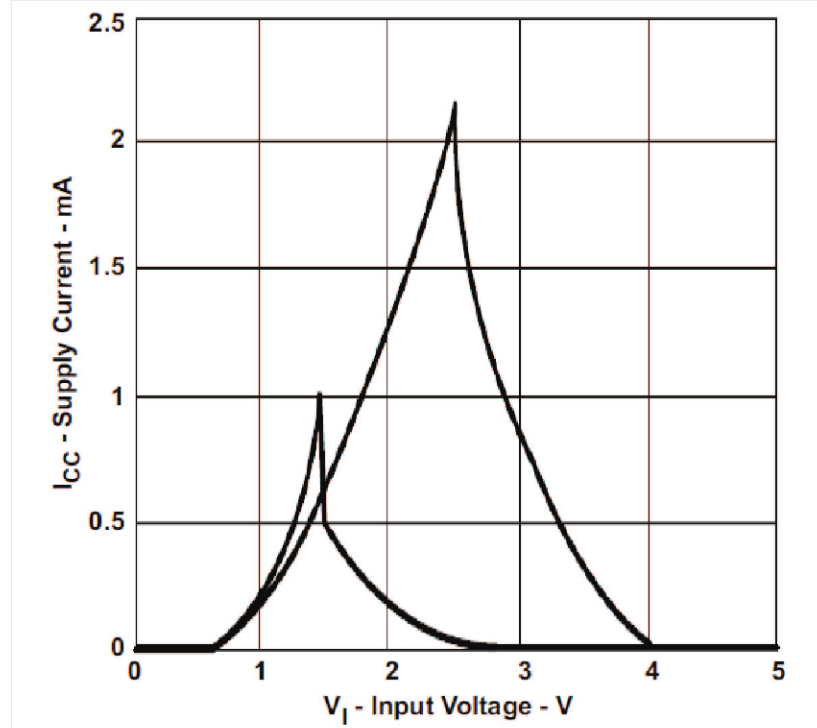
Figure 1. Supply Current vs Input Voltage
