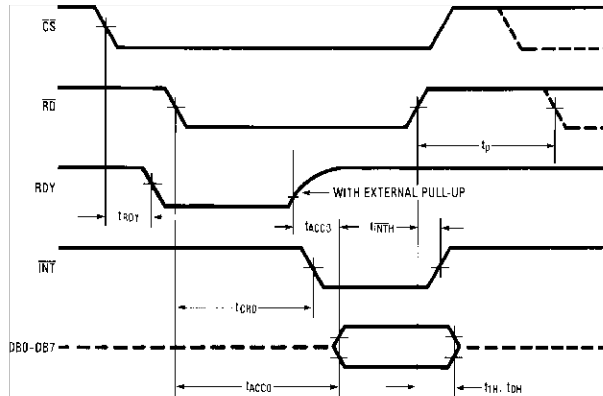
Figure 4. RD Mode (Pin 7 is Low)
