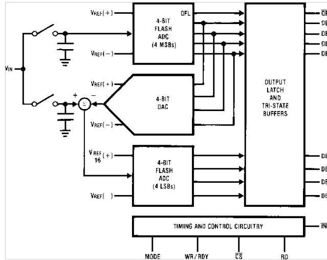
Figure 3. Functional Diagram
