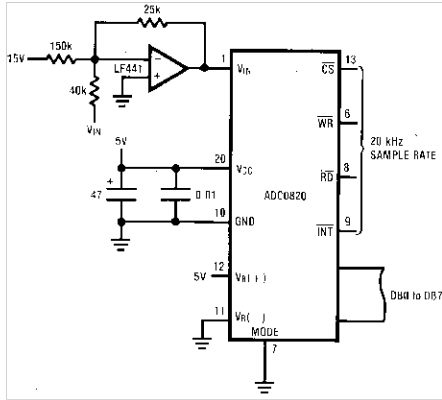
Figure 31. Telecom A/D Converter
