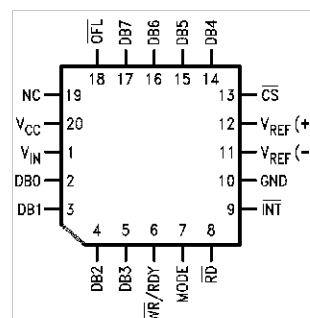
Figure 2. PLCC Package
