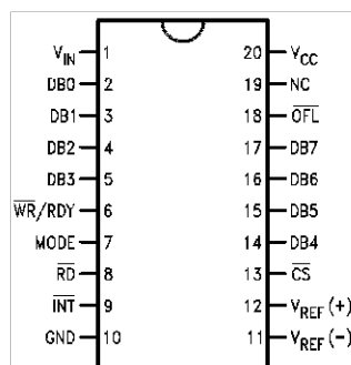
Figure 1. CDIP, PDIP, and SOIC Packages (Top View)
