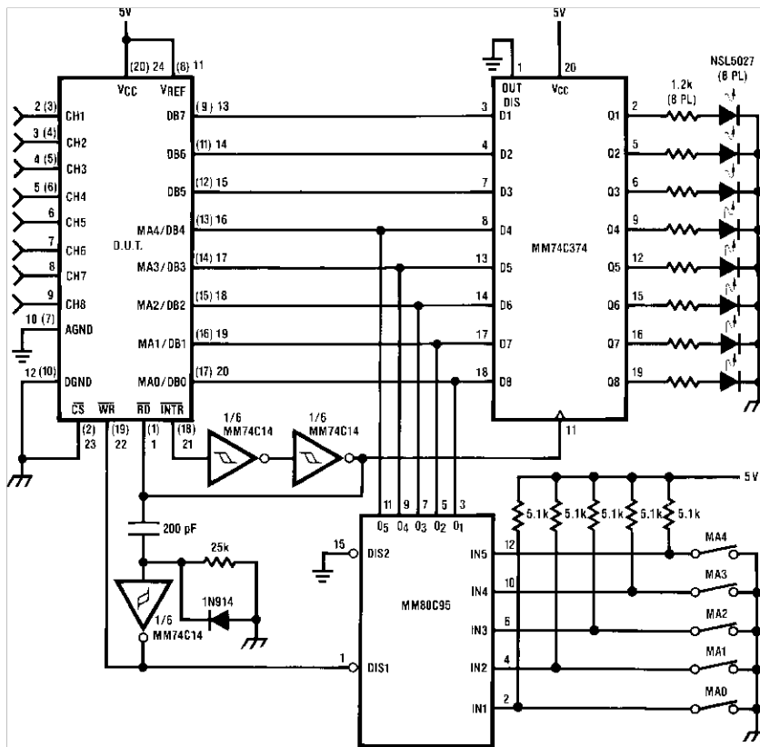
Figure 21. A Stand Alone Circuit
