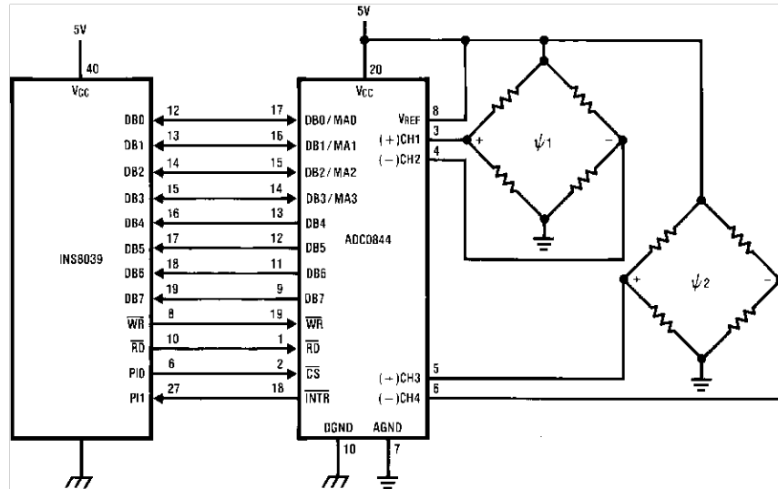
Figure 23. ADC0844—INS8039 Interface
