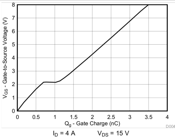
Figure 4. Gate Charge
